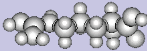
arginine.stl
