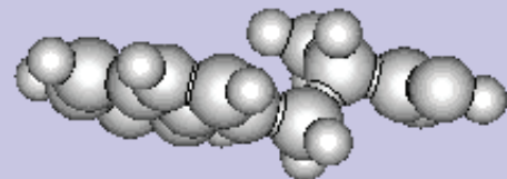
tryptophan.stl
