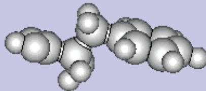
phenylalanine.stl
