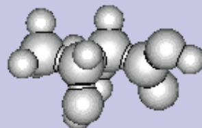
threonine.stl
