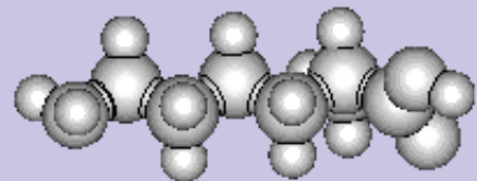
lysine.stl
