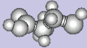
cysteine.stl
