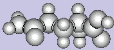
glutamate.stl
