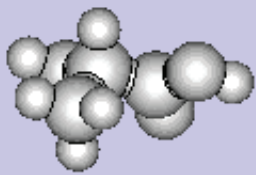
alanine.stl
