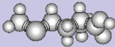
methionine.stl
