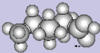
isoleucine.stl
